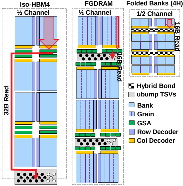
Figure 8: Data movement within bank and channel. FGDRAM layout is adjusted to use a 16 banks per channel configuration. FB-HBM layout shown for a 4-Hi stack for readability.
