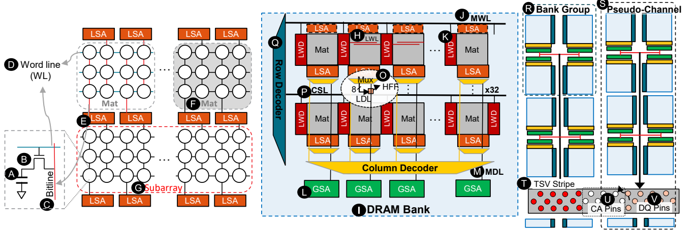
Figure 2: DRAM Organization
