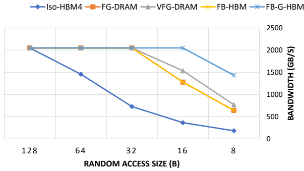
Figure 13: Effective irregular bandwidth for proposed FB-HBM and FB-G-HBM compared against Iso-HBM4, FG-DRAM, and VFG-DRAM for different random access sizes.
