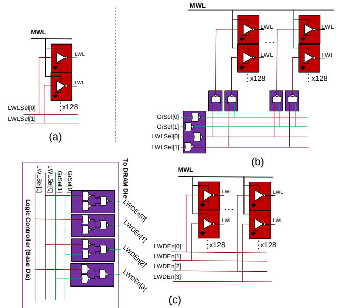
Figure 10: Circuit-level comparison of local wordline drivers: (a) HBM3, (b) FG-DRAM, and (c) FB-G-HBM.
