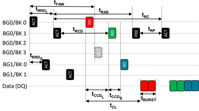
Figure 4: DRAM Timing Constraints
