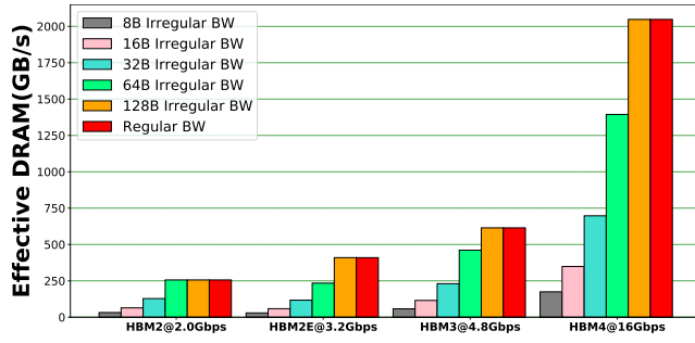
Figure 1: Regular vs. Irregular Bandwidth in HBM
