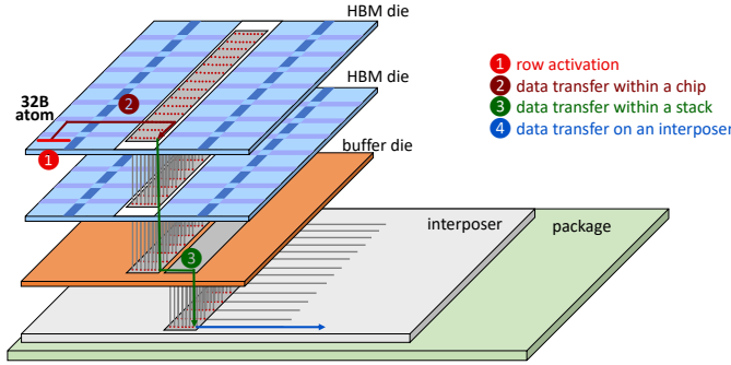
Figure 3: Baseline HBM Stack (from O'Connor et al. [33])
