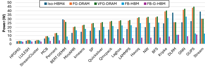
Figure 15: Power for FB-HBM and FB-G-HBM compared against Iso-HBM4, FG-DRAM, and VFG-DRAM.
