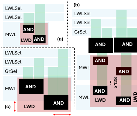
Figure 9: FG-DRAM Area Overhead.
