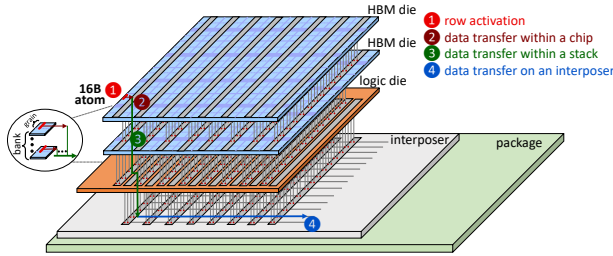
Figure 7: Proposed Folded Banks HBM stack
