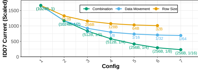
Figure 5: IDD7 (HBM4 estimates) vs. DRAM Config
