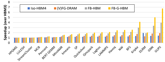
Figure 14: Application speedup over HBM3 for FB-HBM and FB-G-HBM compared against Iso-HBM4 and (V)FG-DRAM.
