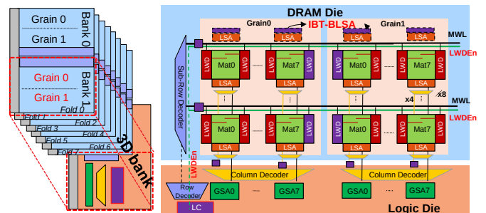
Figure 11: Folded Banks with Small Rows
