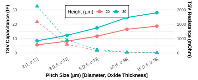
Figure 12: TSV Resistance and Capacitance Sensitivity
