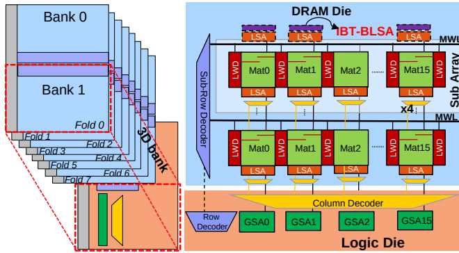
Figure 6: Folded Bank Design
